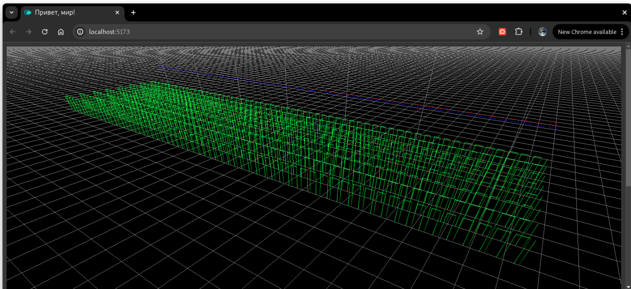
Fig. 5. An example of visualization obtained using Grafix technology. The work of 8 work processes is shown. Time goes from left to right. Workers are located each on their own Z axis (closer to and further from the screen). The horizontal line on the worker axis is the task execution. The vertical line is the worker receiving input data from the master and sending him the result. In the background, the blue segments are the master waiting for all the workers, the red ones are the master estimating the current situation.
